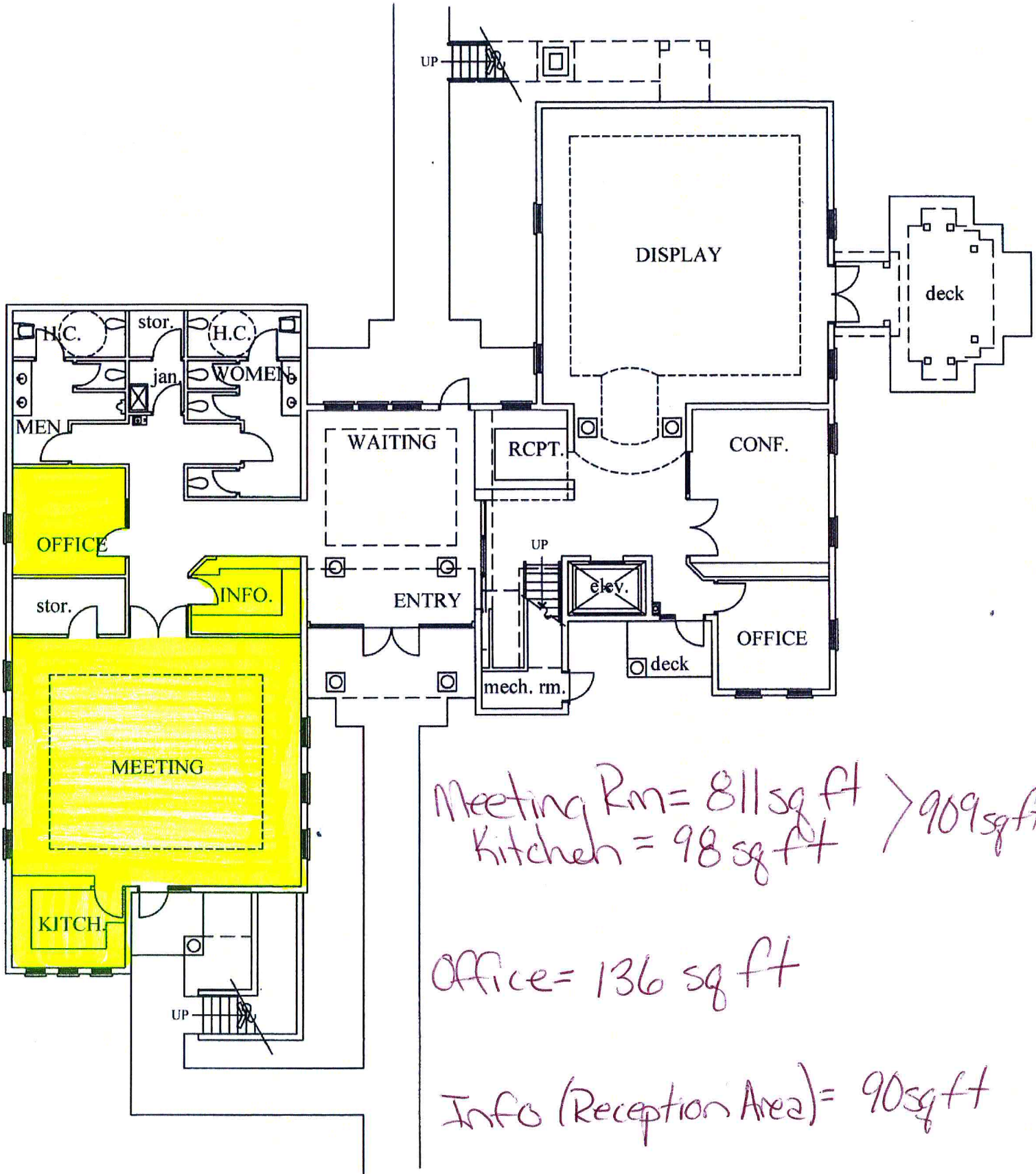
1st FLOOR PLAN 1/8" = 1' - 0"
